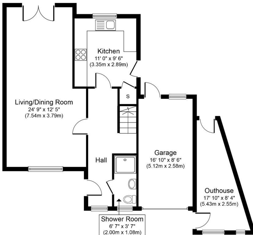
Ground Floor Approximate Floor Area 688 sq. ft. (63.9 sq. m.)
